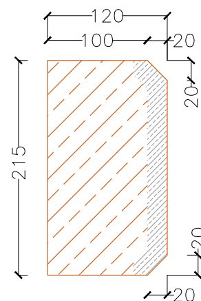
LQ3 & LQ4 Section
