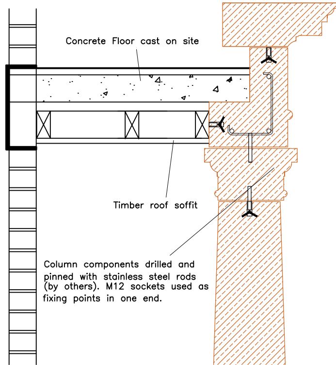
Typical Fixing Detail
