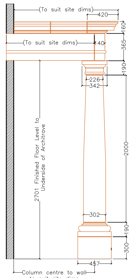
Portico - Side Elevation.
