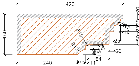
Cornice Section
