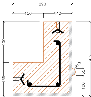
Architrave Section
