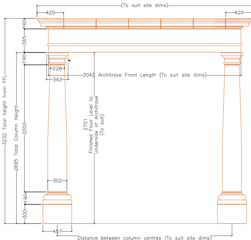
Portico - Front Elevation.
