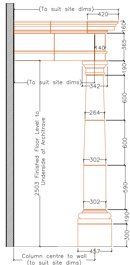
Portico - Side Elevation.
