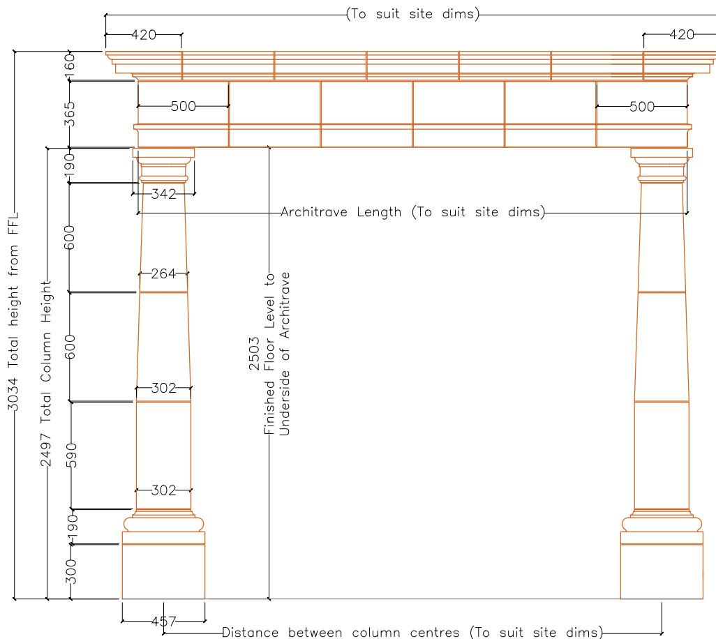
Portico - Front Elevation.
