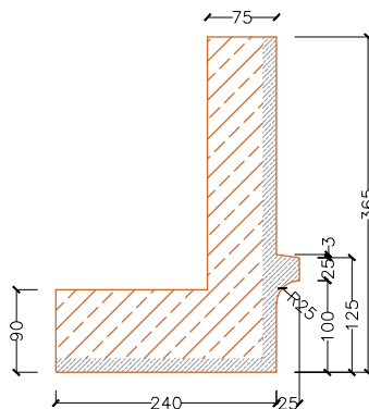
Architrave Section
