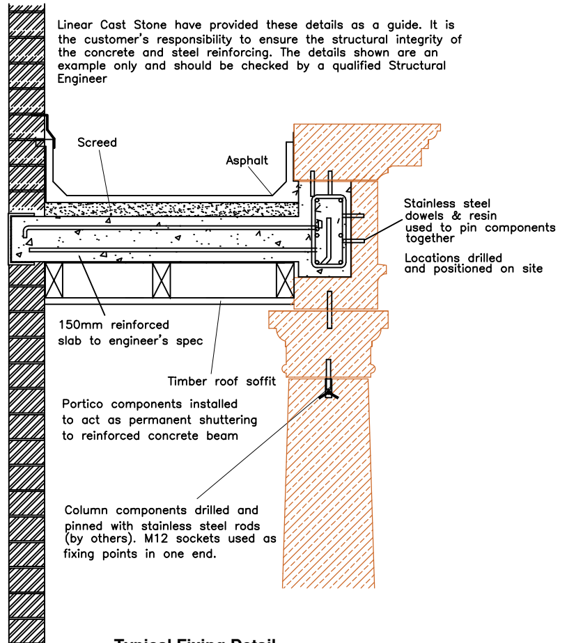
Typical Fixing Detail
