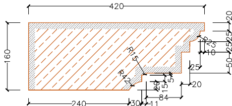
Cornice Section
