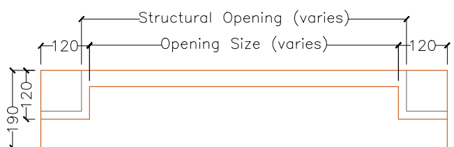
LC2 - Plan (To Render)
