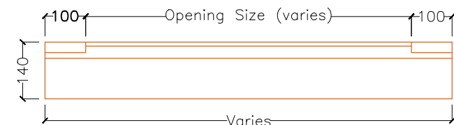
LC1 - Elevation (To Brickwork)
