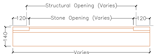
LC2 - Elevation (To Render)
