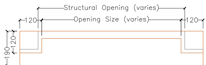
LC4 - Plan (To Render)
