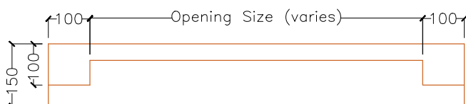
LC3 - Plan (To Brickwork)
